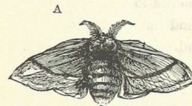
A. THE BOMBYX MORI MOTH. B. ITS COCOON. C. THE OLEANTHUS MOTH.
